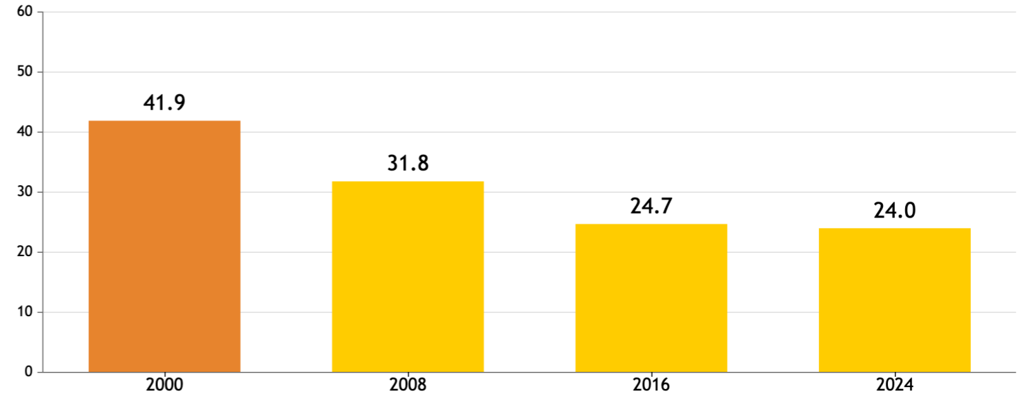
GHI Score Trend for Mali
