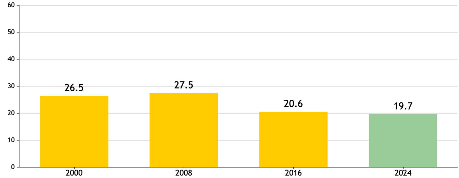
GHI Score Trend for Namibia
