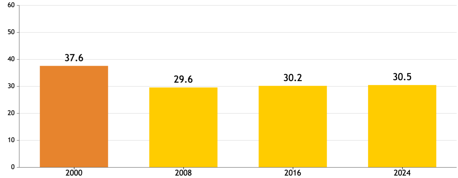
GHI Score Trend for Guinea-Bissau
