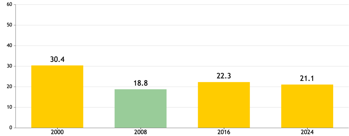
GHI Score Trend for Mauritania
