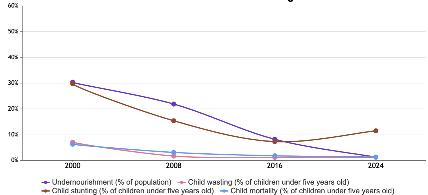
Trend for Indicator Values - Mongolia
